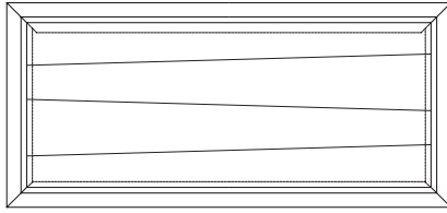
Upholstered King Headboard SKU #120-727 78" w x 1-7/8" d x 36" h
