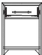
Nightstand SKU #120-300 22" w x 16" d x 28" h
